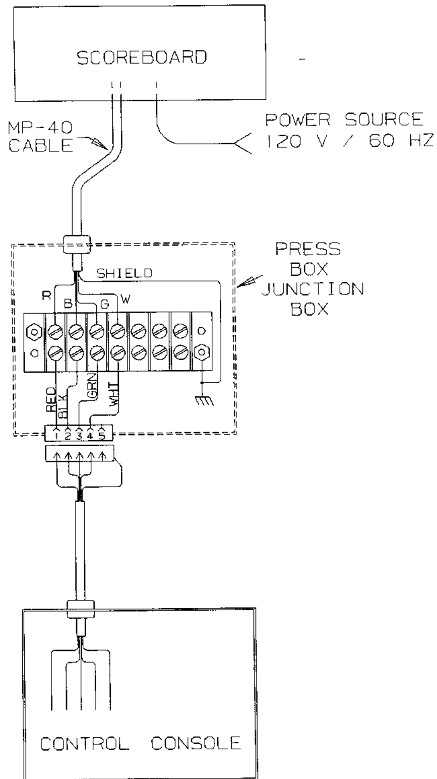
figure 4 SYSTEM LAYOUT
