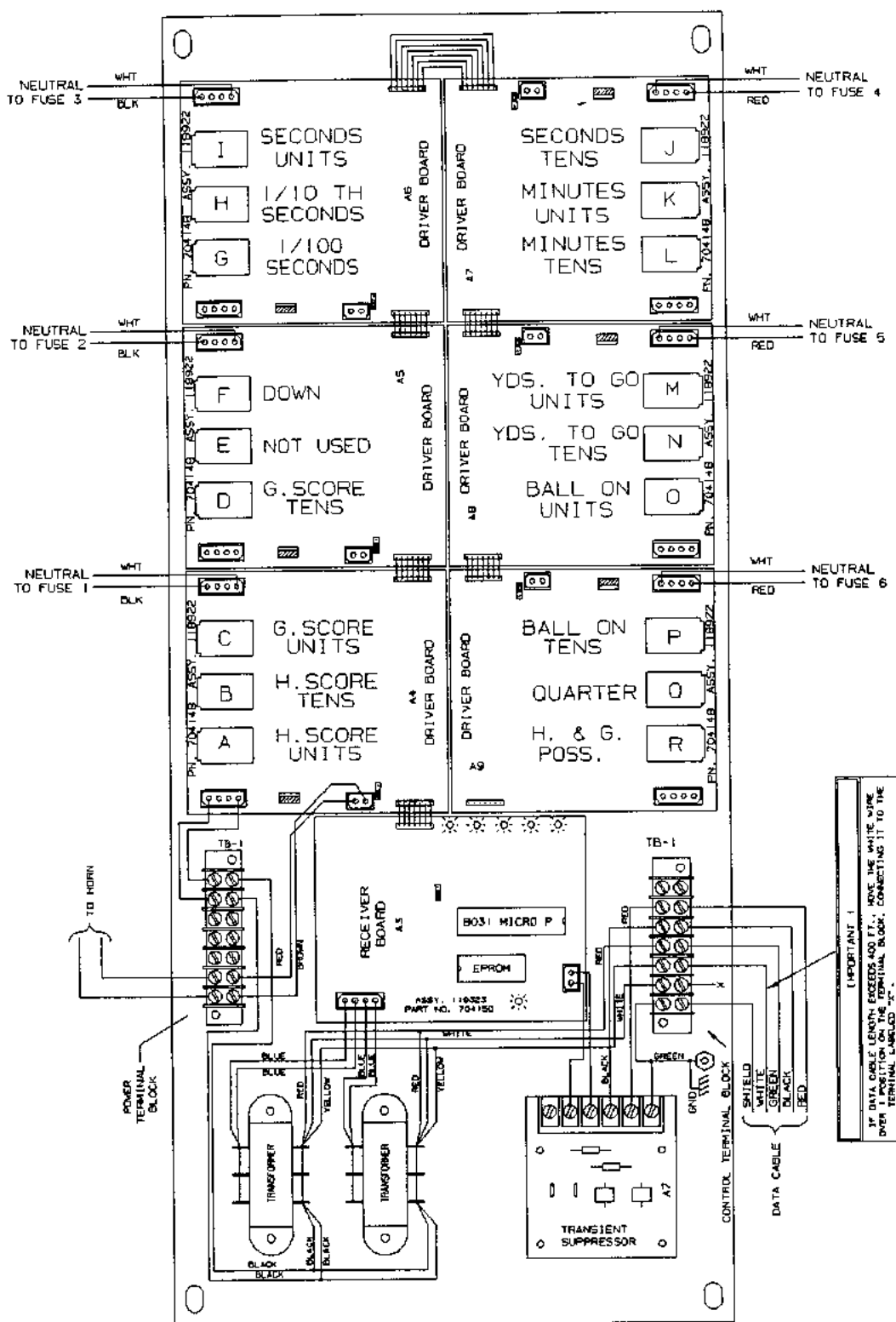
CONTROLLER ASSEMBLY
