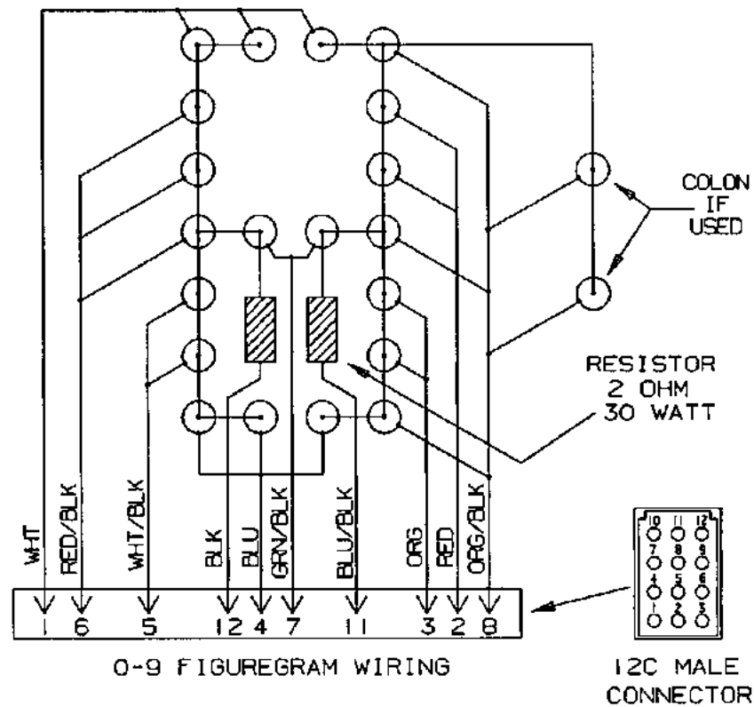
FIGUREGRAM WIRING
