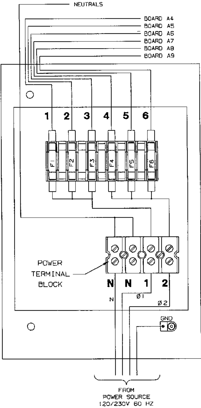
POWER WIRING
